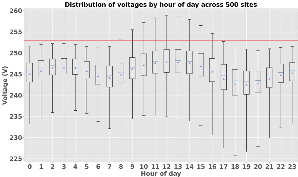
Figure 13 Distribution of voltages from Solar Analytics sites over 24h
