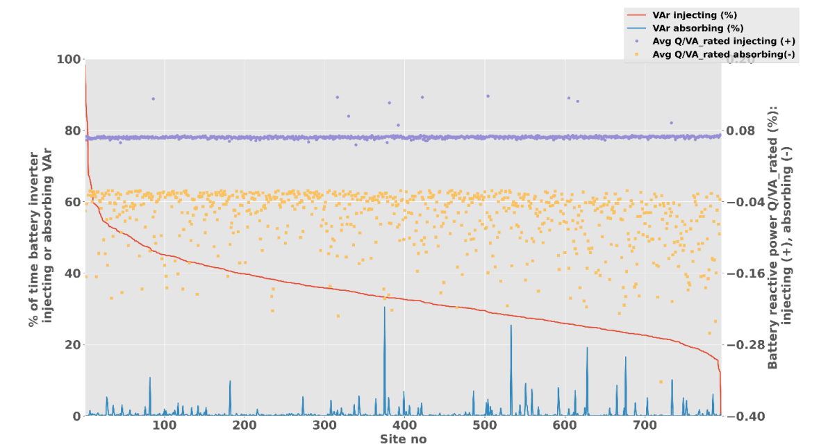
Figure 21 Percentage of time BESS is injecting or absorbing VARs (left y axis) and average rate of VAR injection or absorption (right-axis) ordered by the percentage of injecting VARs
